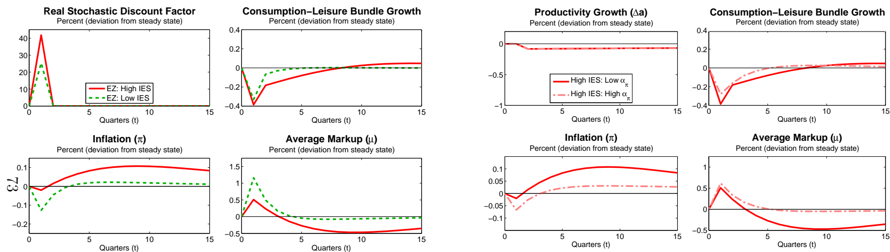
Fig. A2: Negative Long-Run Shock
