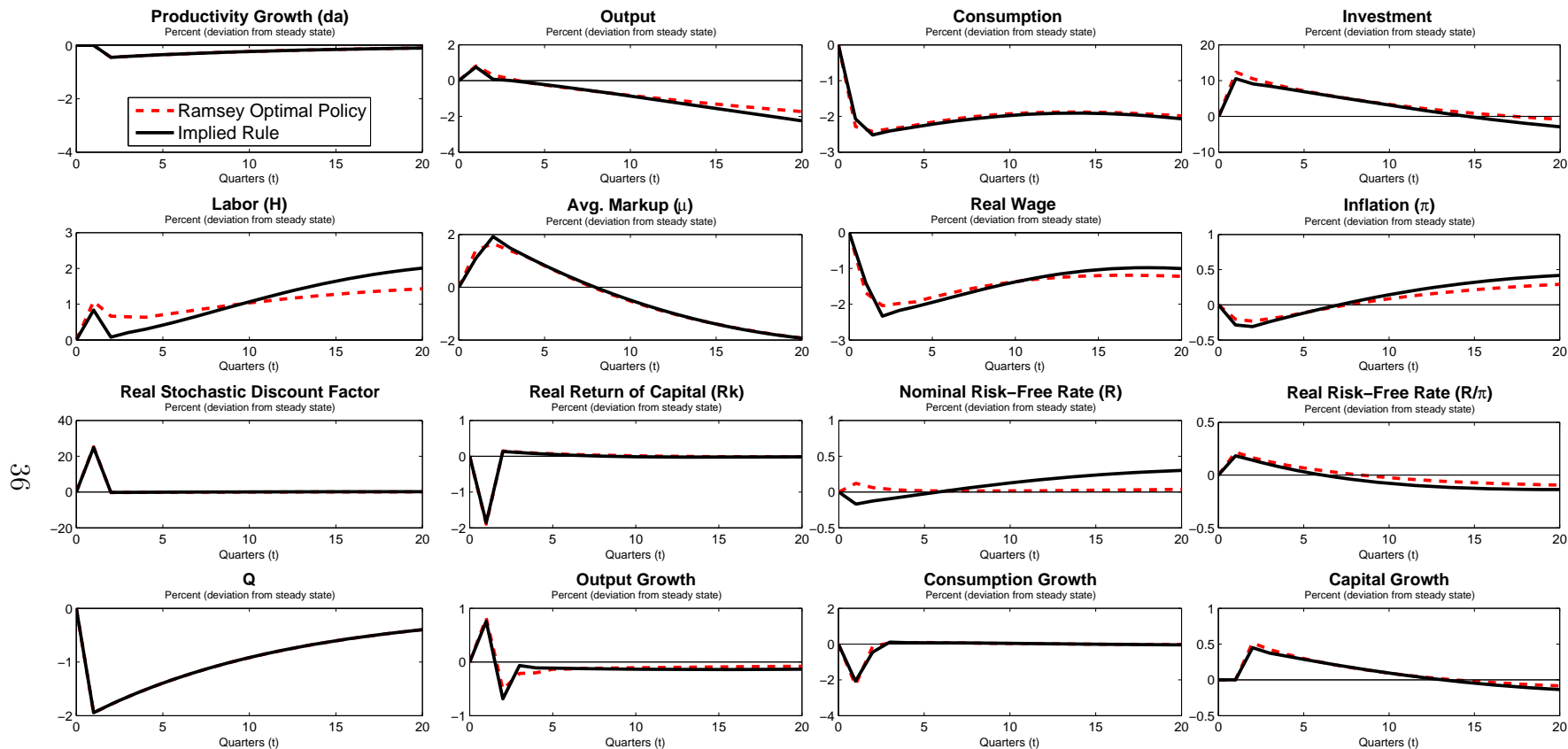
Fig. 8: Ramsey Optimal Monetary Policy and Implied Rule: Negative Long-Run Shock
