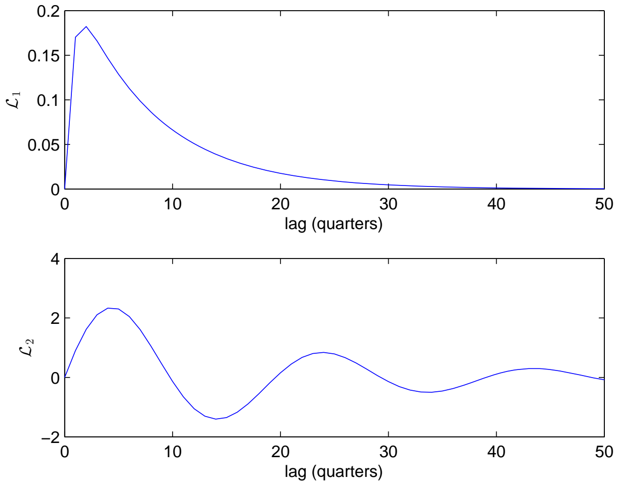
Figure 3: Impulse response for overvaluation. The top panel plots \{\mathcal{L}_1(j)\}_{j \geq 0} for lag j = 0, 1, \dots, 50 . The bottom panel plots \{\mathcal{L}_2(j)\}_{j \geq 0} for lag j = 0, 1, \dots, 50 . The parameters are \theta = 0.9 , \mu_0 = 0.3 , and \bar{w} = 0.1 .
