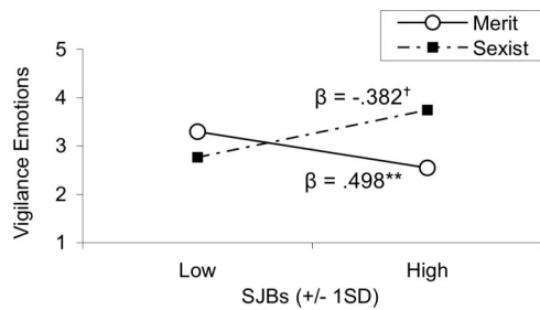
Figure 4. Preinteraction feelings of vigilance. Condition (merit = 0, sexist = 1) \times SJBs (continuous, mean-centered) interaction. Graphed at \pm 1 SD from SJBs mean. SJB = system-justifying beliefs. \dagger p \leq .10 . * p < .05 .
