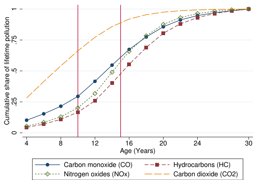
Figure 7: Cumulative Share of Fleet Emissions from Each Vehicle Age
