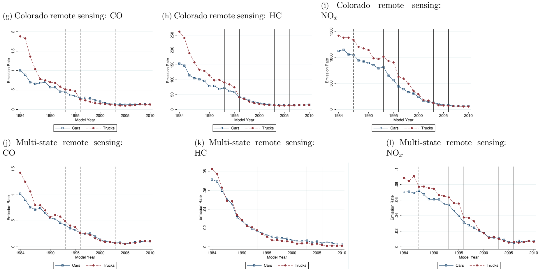
Figure A3: Exhaust Standards and Emission Rates, Cars Versus Trucks
