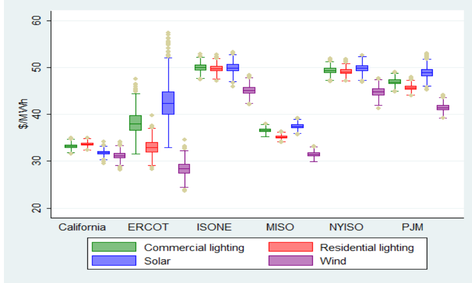
Figure 5: Avoided operating costs per MWh by technology type and region.
