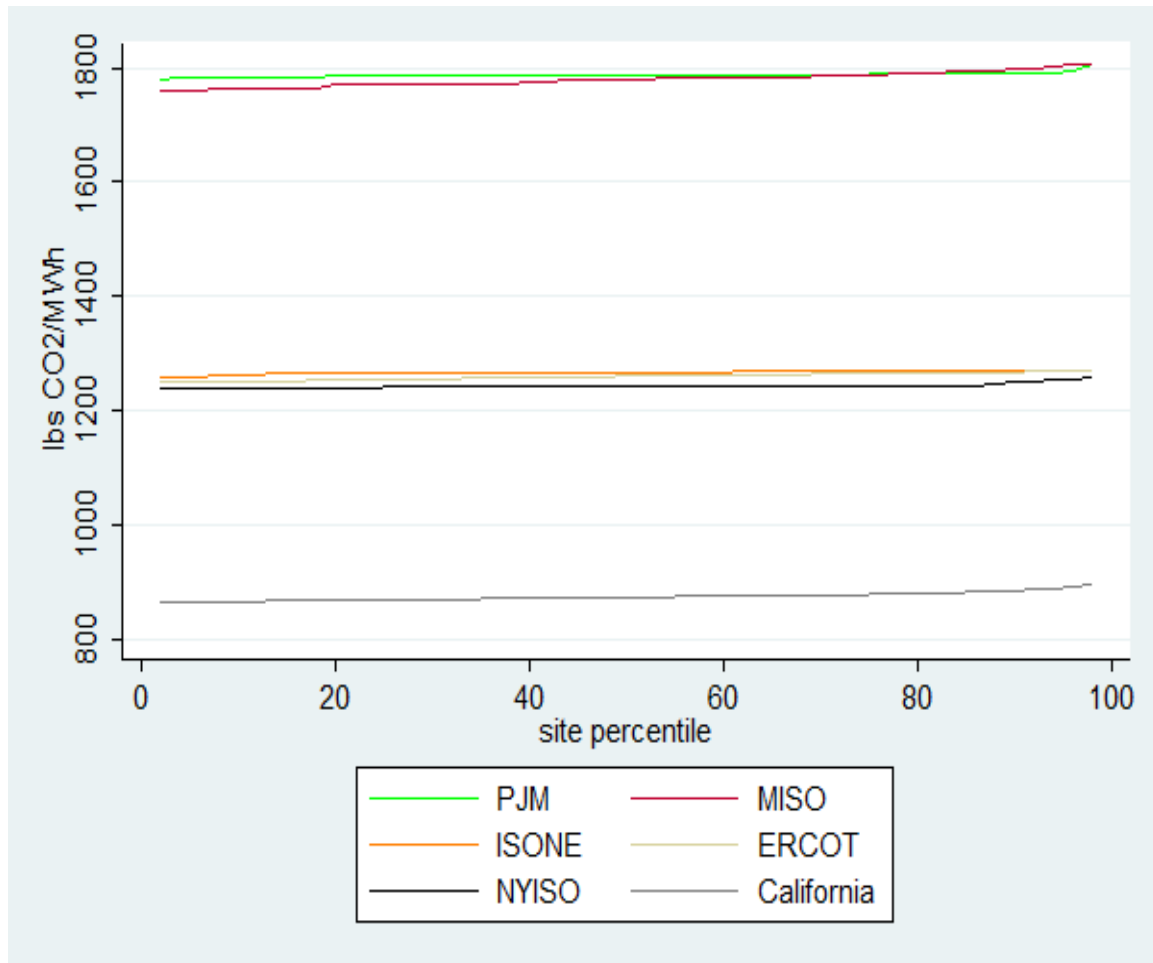
Figure 15: Site-specific marginal emissions displacement
