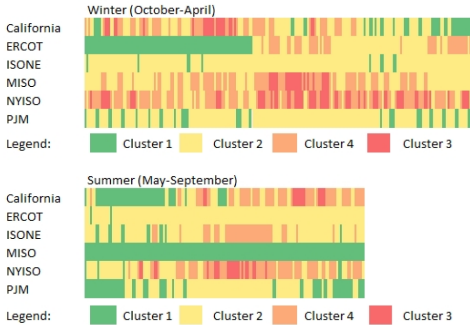
Figure 13: Cluster composition over the time period
