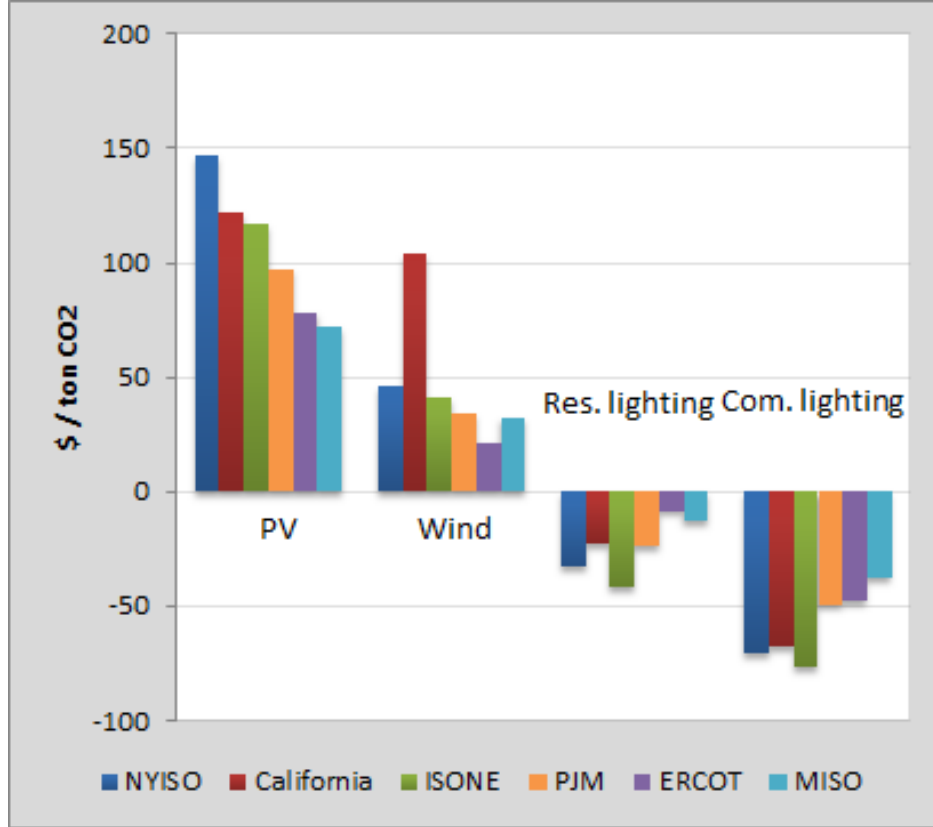
Figure 7: Marginal abatement costs across technologies and regions
