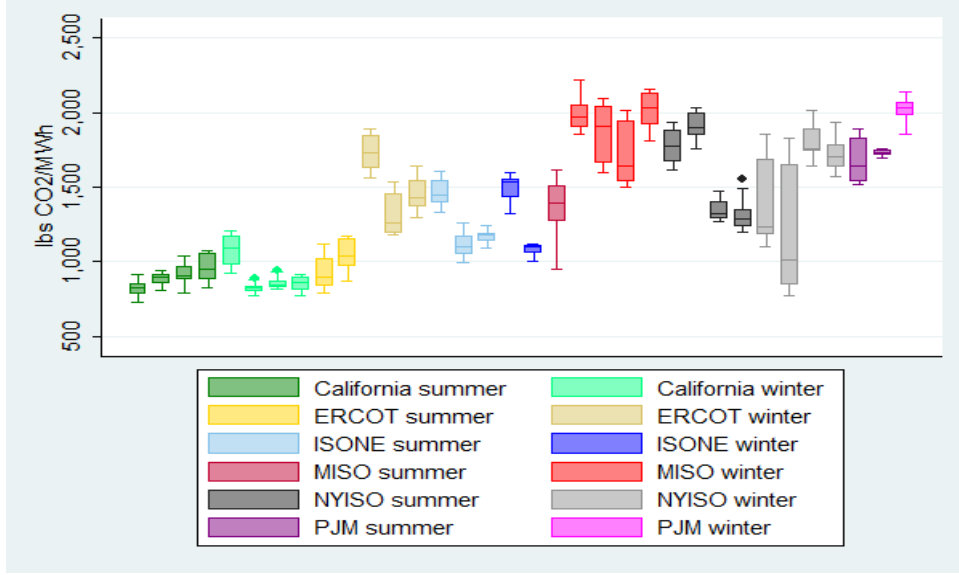
Figure 3: Seasonal marginal operating emissions rates
