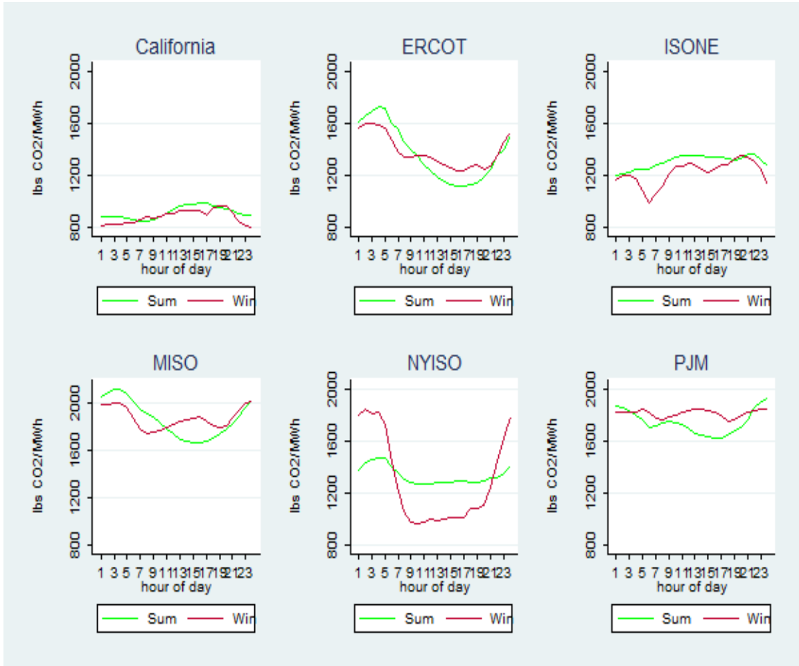
Figure 14: Marginal operating emissions rates
