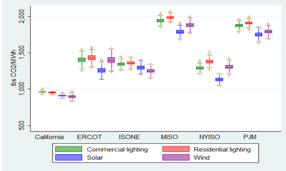
Figure 4: Marginal emissions displacement rates
