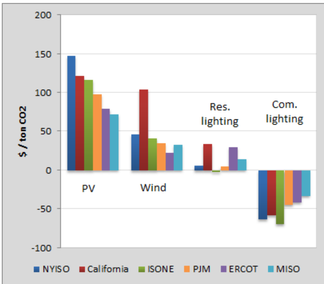
Figure 16: Marginal abatement costs at 50% energy efficiency realization rate
