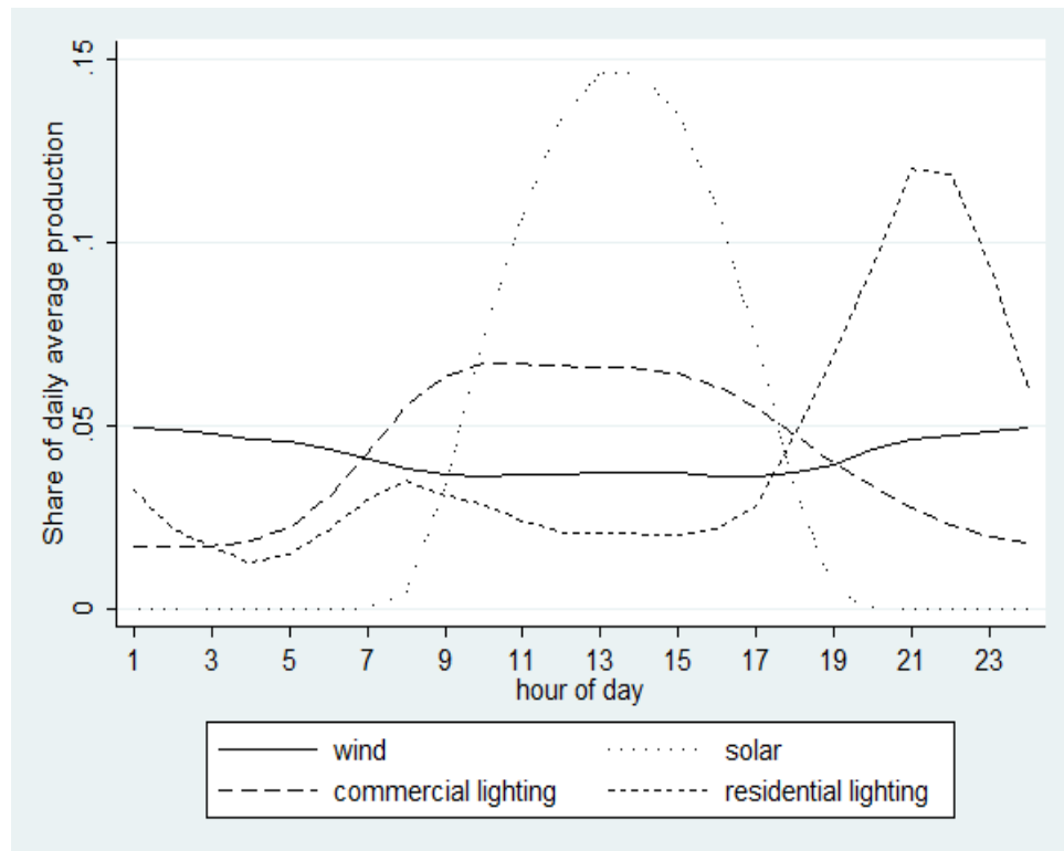
Figure 2: Resource-specific production profiles
