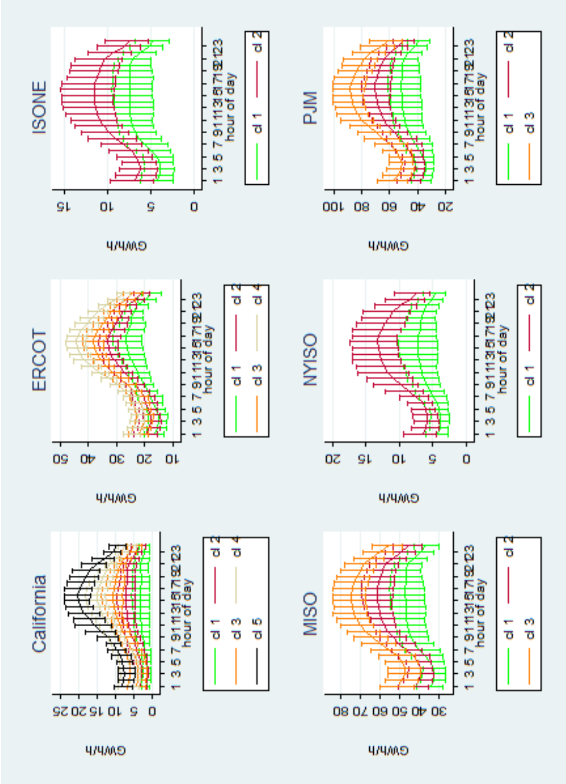
Figure 11: K-means clustering: Summer generation profiles
