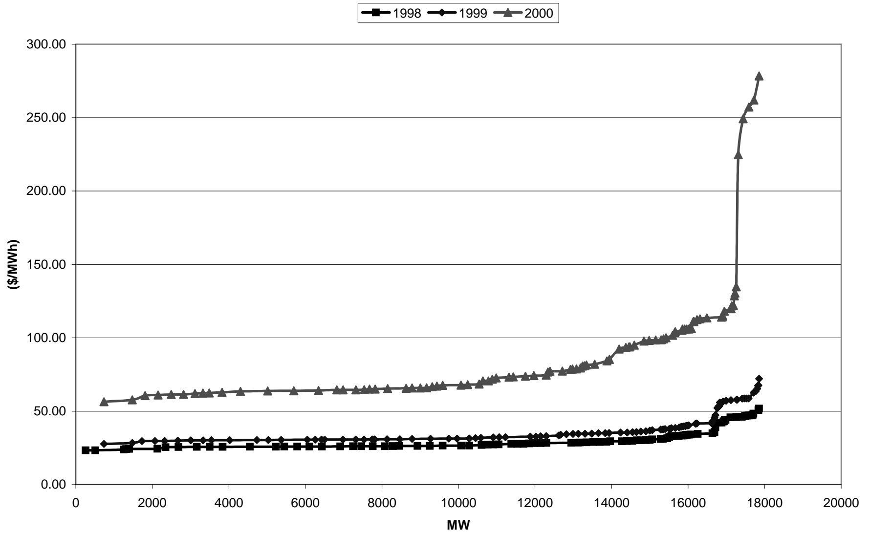
Figure 1: California Fossil Plant MC Curves (September)
