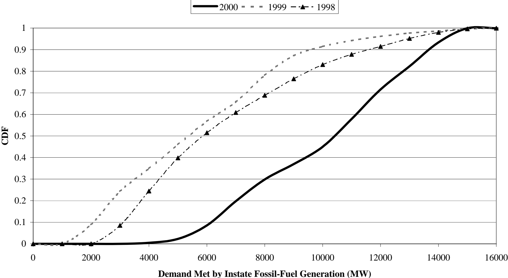
Figure 4: Cumulative Distribution Functions of Demand Met by Instate Fossil-Fuel Generation August 7 - September 30
